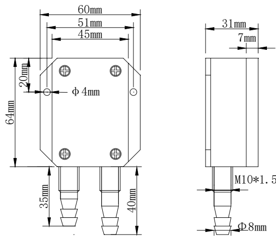
Φ (8) interface dimension drawing of pagoda mouth
