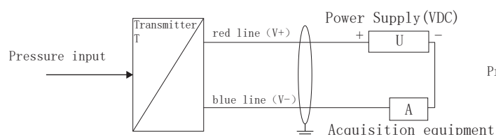
Current output wiring diagram (two-wire system)
