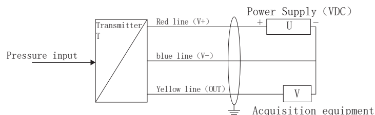
Voltage output wiring diagram (three wire system)
