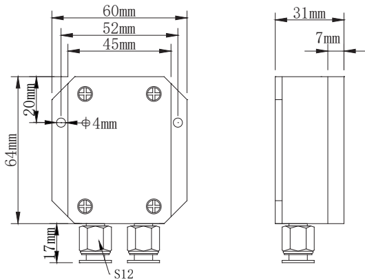
Φ (6) dimension drawing of quick interface
