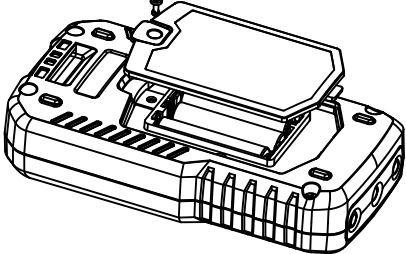
Open the battery cover
